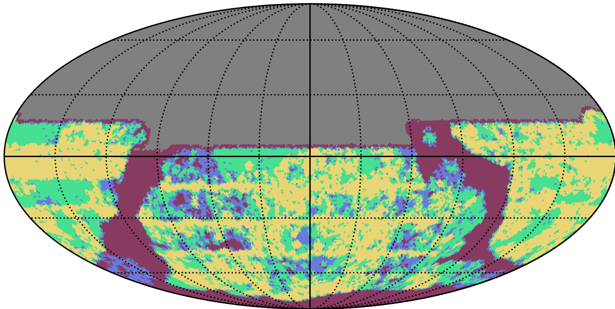
baseline_v3.4_10yrs u band: YearCoverage night
