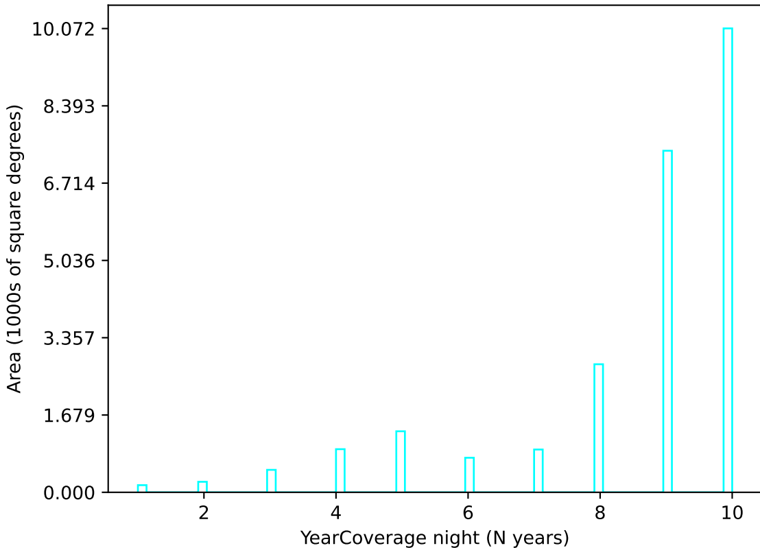
baseline_v3.4_10yrs u band: YearCoverage night
