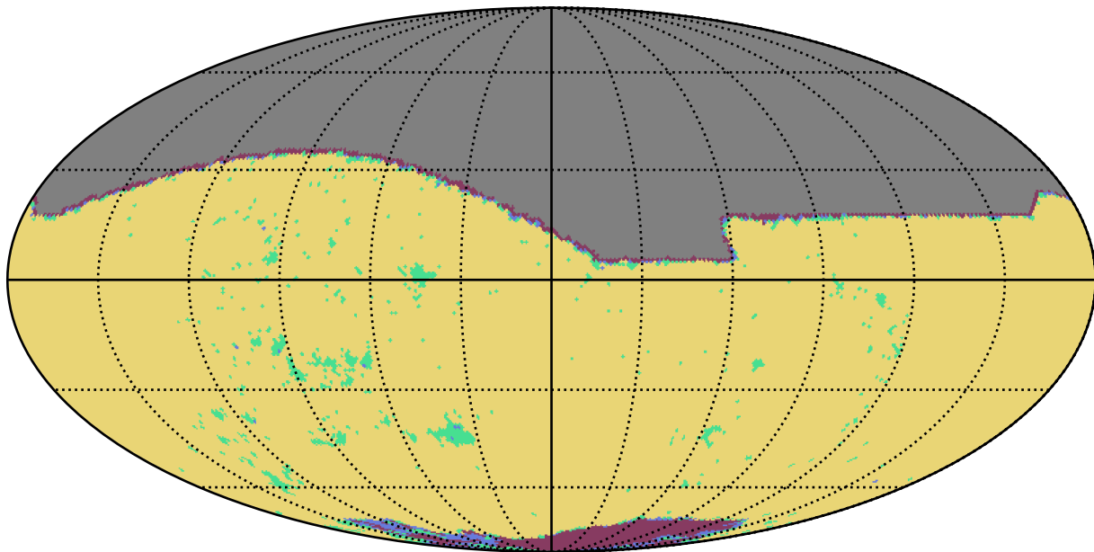
baseline_v3.4_10yrs r band: YearCoverage night
