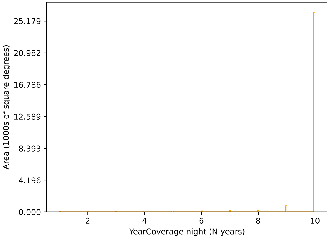
baseline_v3.4_10yrs r band: YearCoverage night
