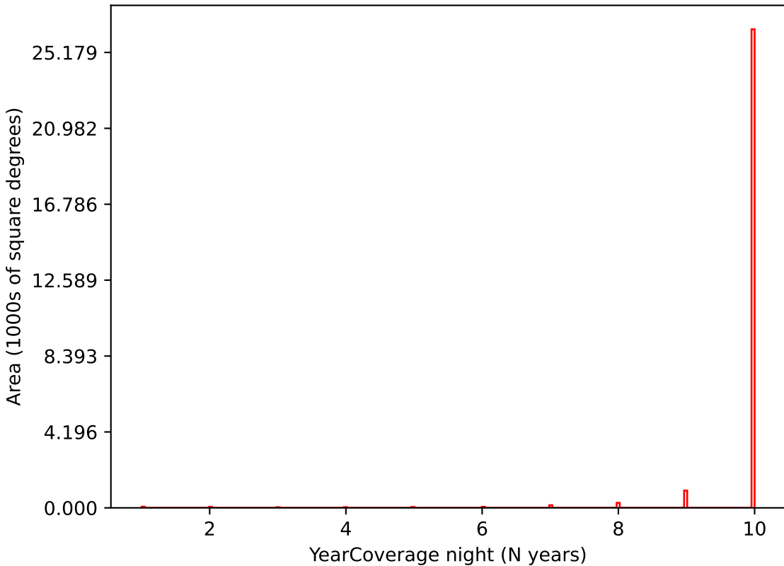
baseline_v3.4_10yrs i band: YearCoverage night
