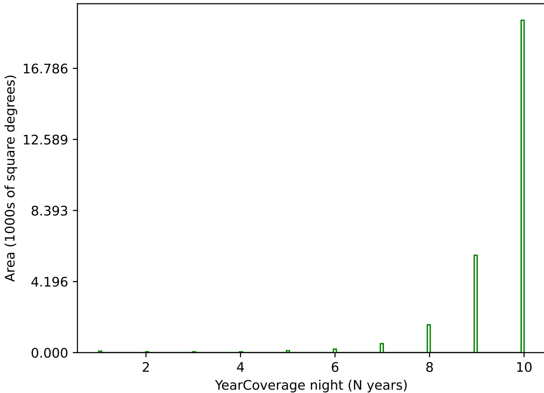
baseline_v3.4_10yrs g band: YearCoverage night
