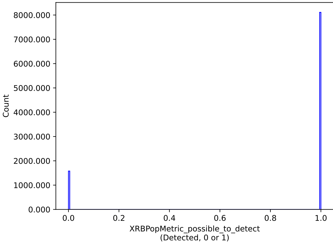
baseline_v3.4_10yrs : XRBPoMetric_possible_to_detect
