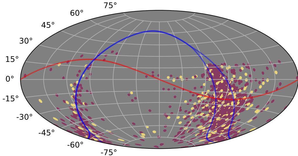
baseline_v3.4_10yrs : XRBPpopMetric_early_detect
