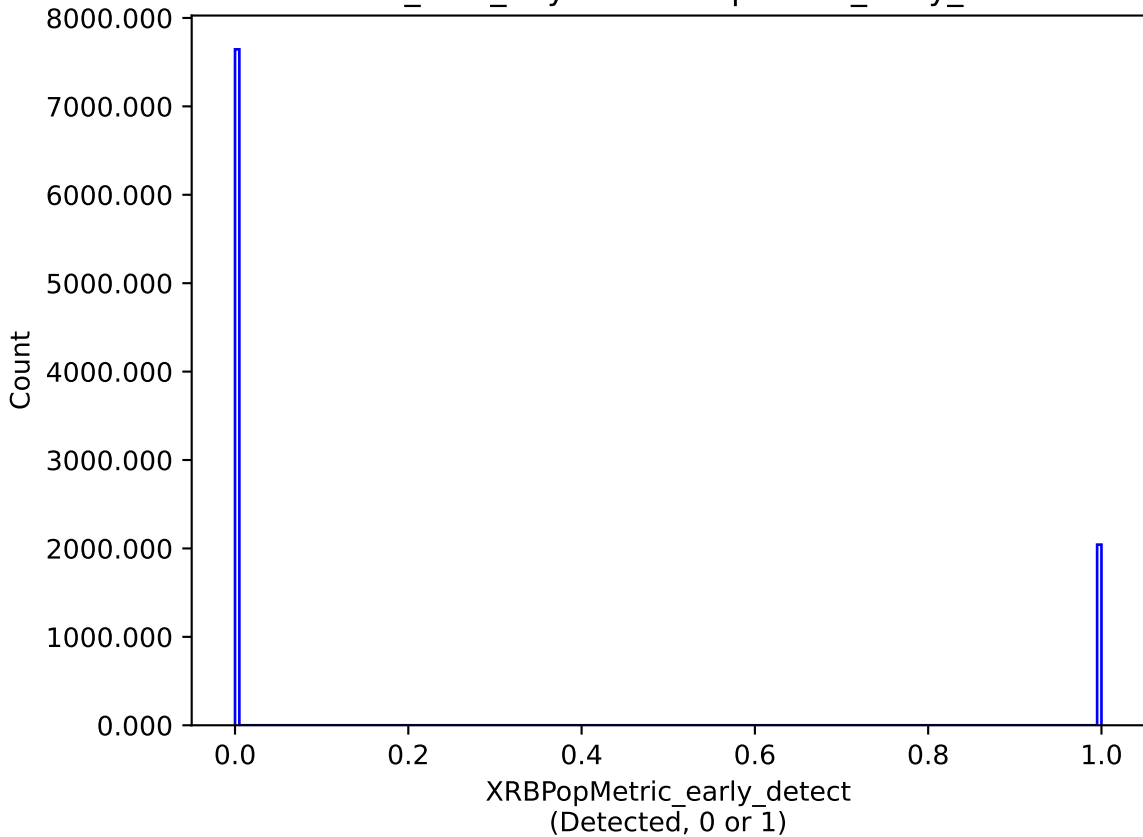
baseline_v3.4_10yrs : XRBPoMetric_early_detect
