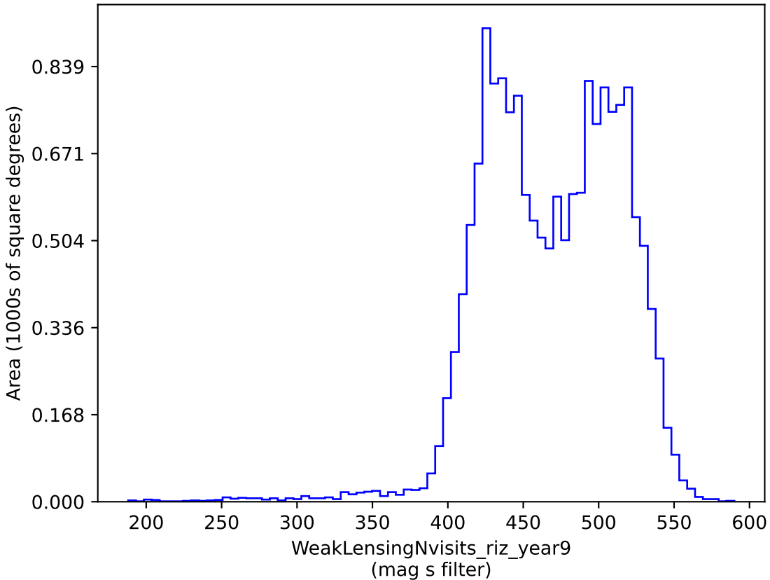
baseline_v3.4_10yrs gri band non-DD: WeakLensingNvisits_riz_year9
