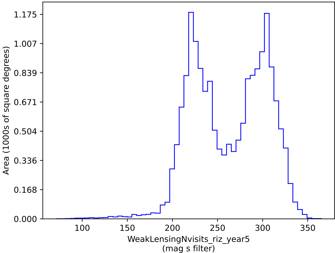
baseline_v3.4_10yrs gri band non-DD: WeakLensingNvisits_riz_year5
