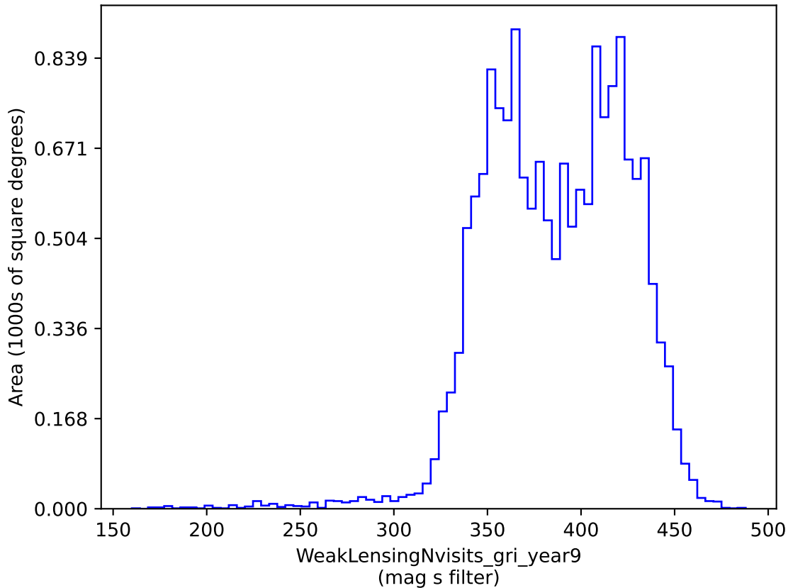
baseline_v3.4_10yrs gri band non-DD: WeakLensingNvisits_gri_year9
