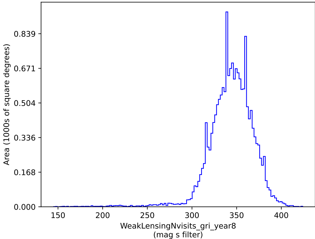
baseline_v3.4_10yrs gri band non-DD: WeakLensingNvisits_gri_year8
