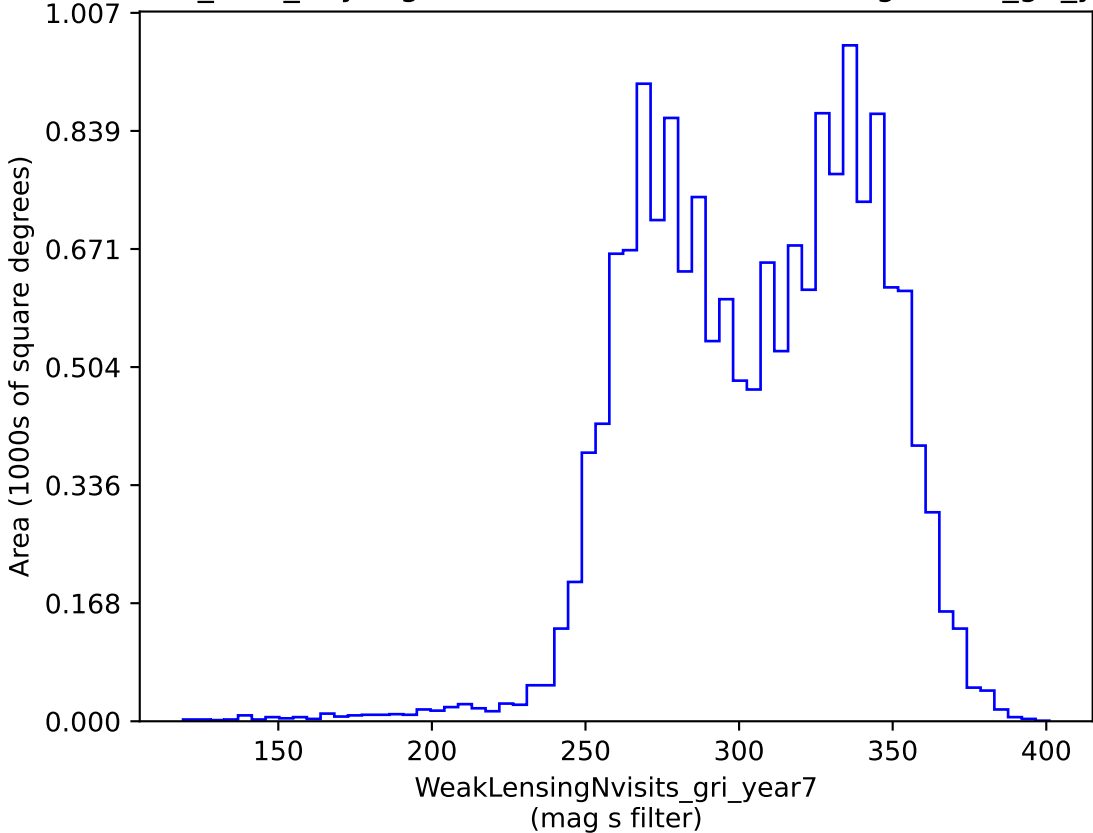
baseline_v3.4_10yrs gri band non-DD: WeakLensingNvisits_gri_year7
