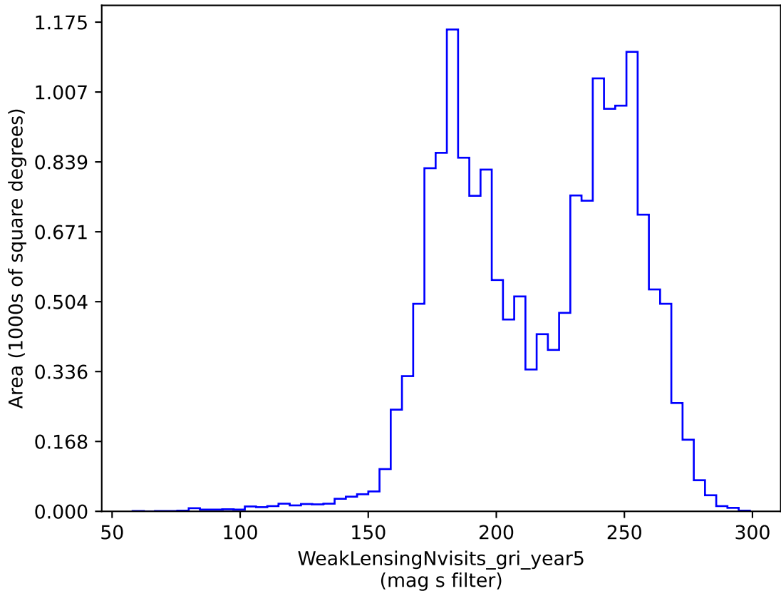
baseline_v3.4_10yrs gri band non-DD: WeakLensingNvisits_gri_year5
