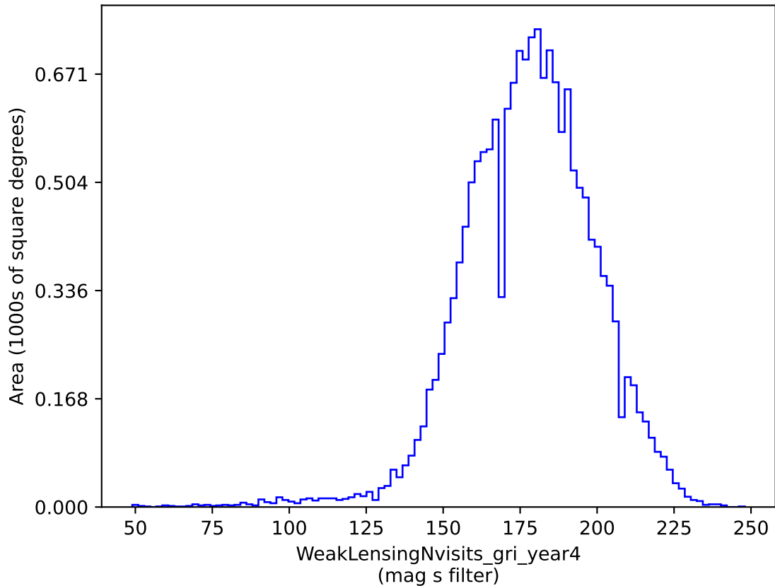
baseline_v3.4_10yrs gri band non-DD: WeakLensingNvisits_gri_year4
