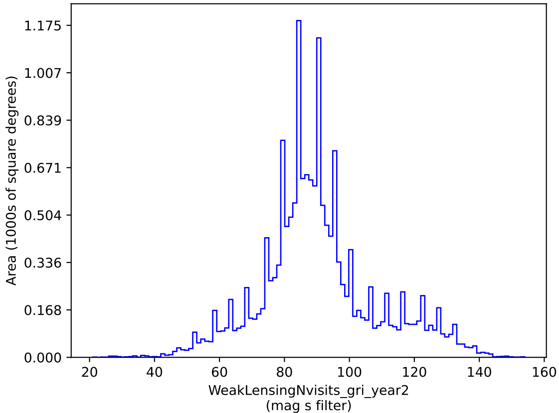
baseline_v3.4_10yrs gri band non-DD: WeakLensingNvisits_gri_year2
