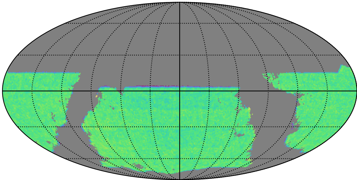
baseline_v3.4_10yrs gri band non-DD: WeakLensingNvisits
