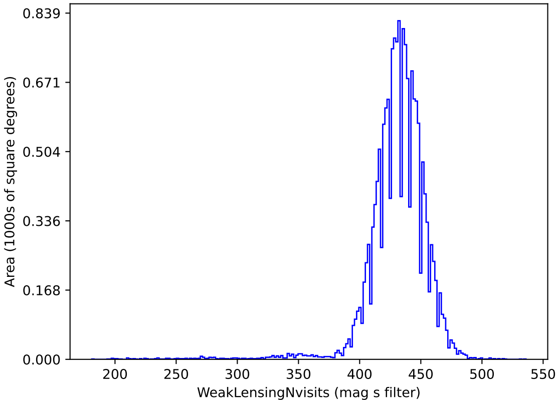
baseline_v3.4_10yrs gri band non-DD: WeakLensingNvisits
