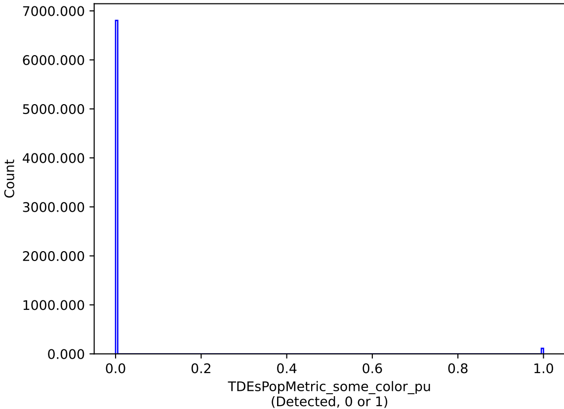
baseline_v3.4_10yrs : TDEsPopMetric_some_color_pu
