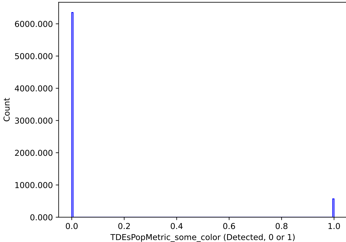
baseline_v3.4_10yrs : TDEsPopMetric_some_color
