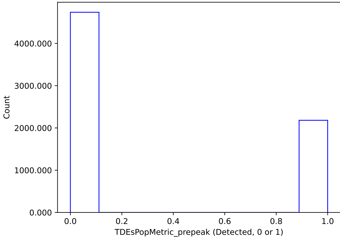
baseline_v3.4_10yrs : TDEsPopMetric_prepeak
