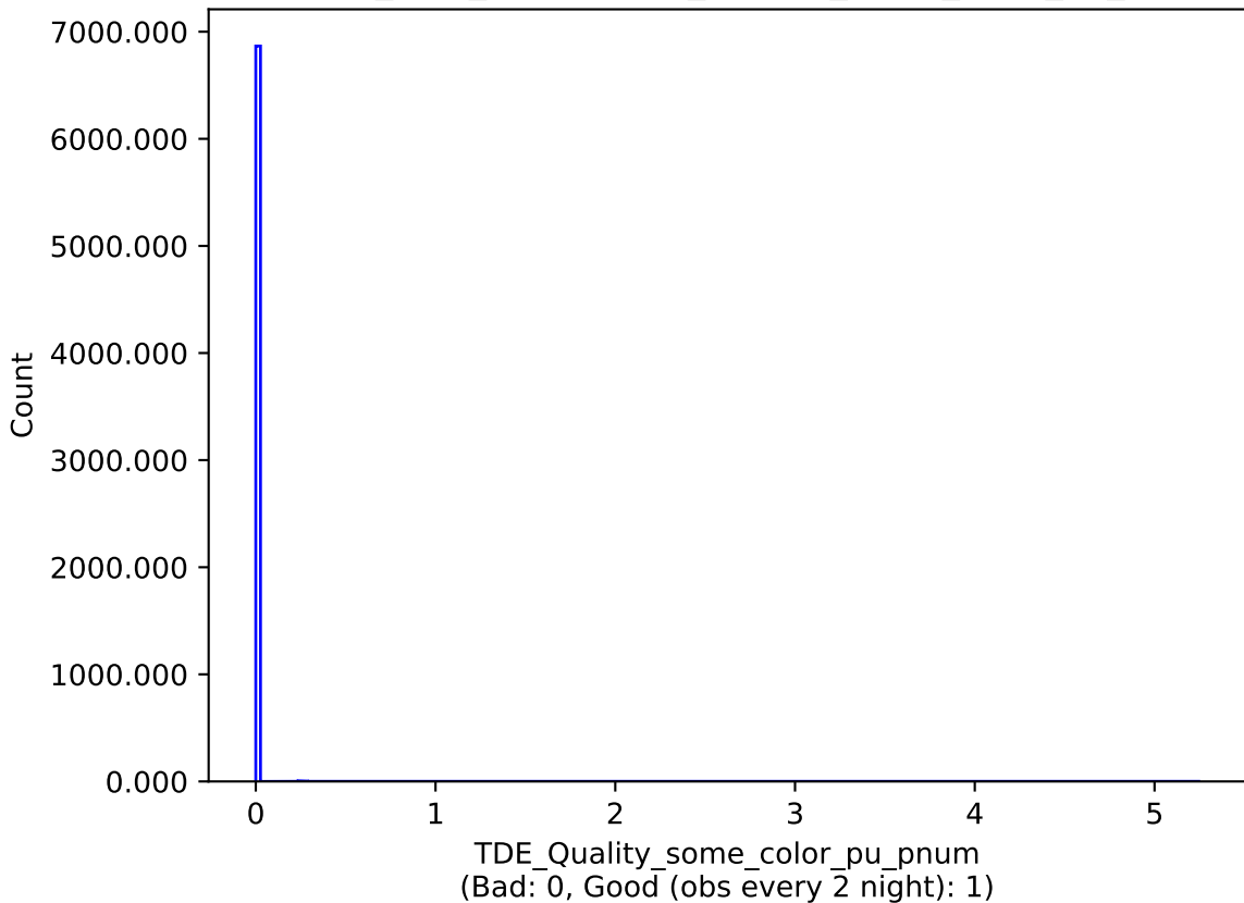
baseline_v3.4_10yrs : TDE_Quality_some_color_pu_pnum
