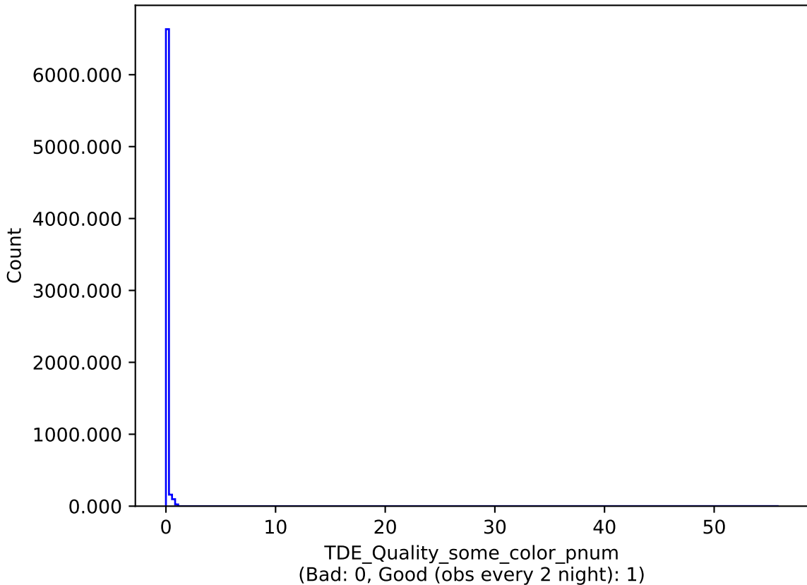
baseline_v3.4_10yrs : TDE_Quality_some_color_pnum
