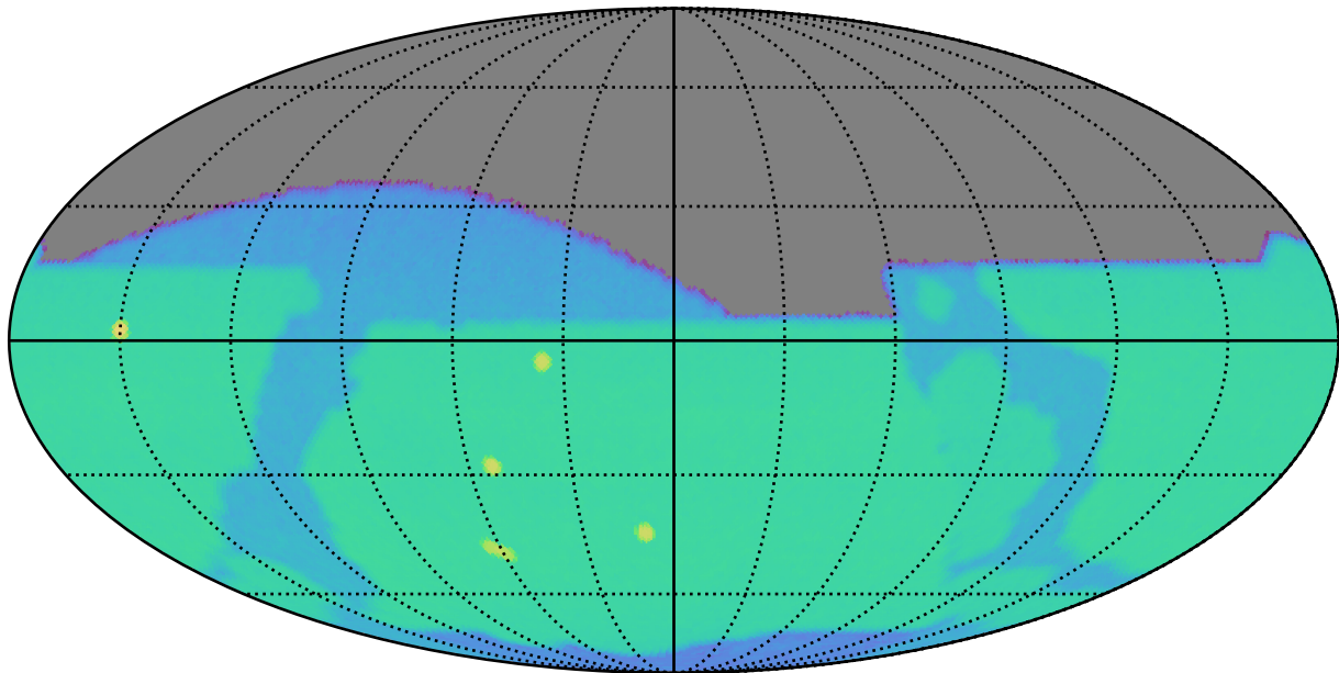
baseline_v3.4_10yrs z: SurfaceBrightLimit
