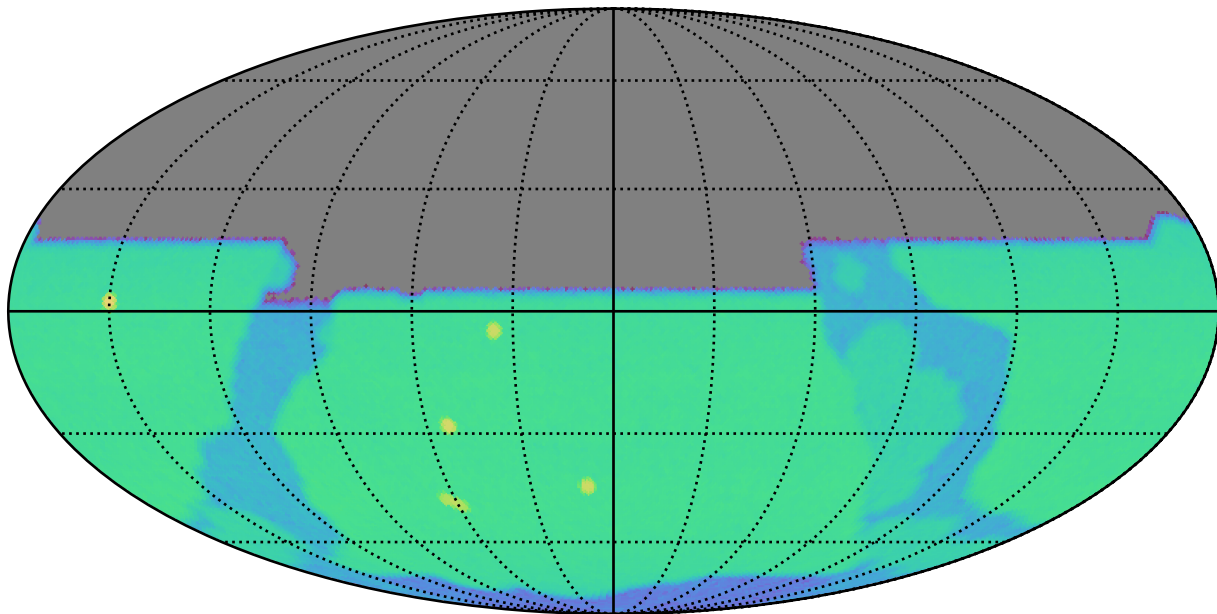
baseline_v3.4_10yrs y: SurfaceBrightLimit
