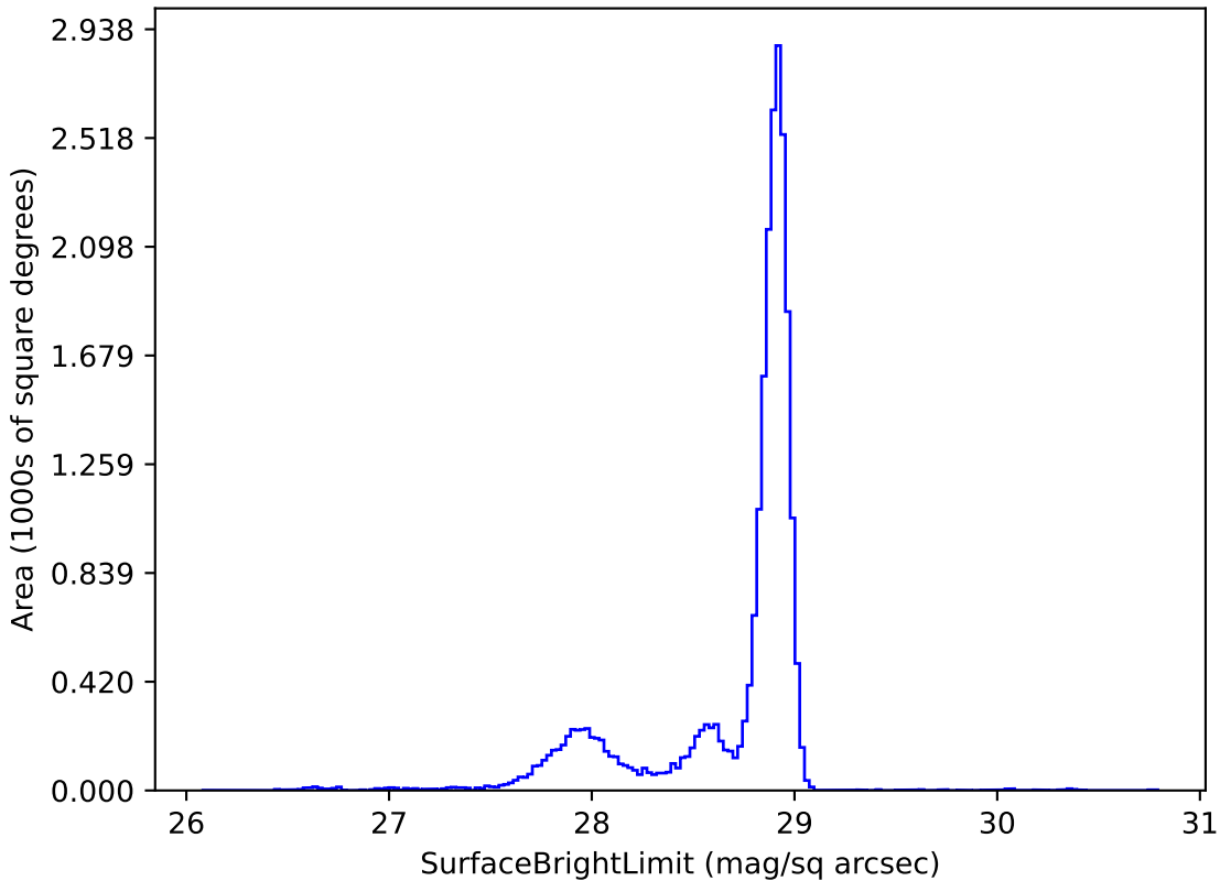
baseline_v3.4_10yrs u: SurfaceBrightLimit
