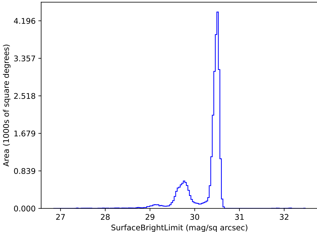
baseline_v3.4_10yrs r: SurfaceBrightLimit
