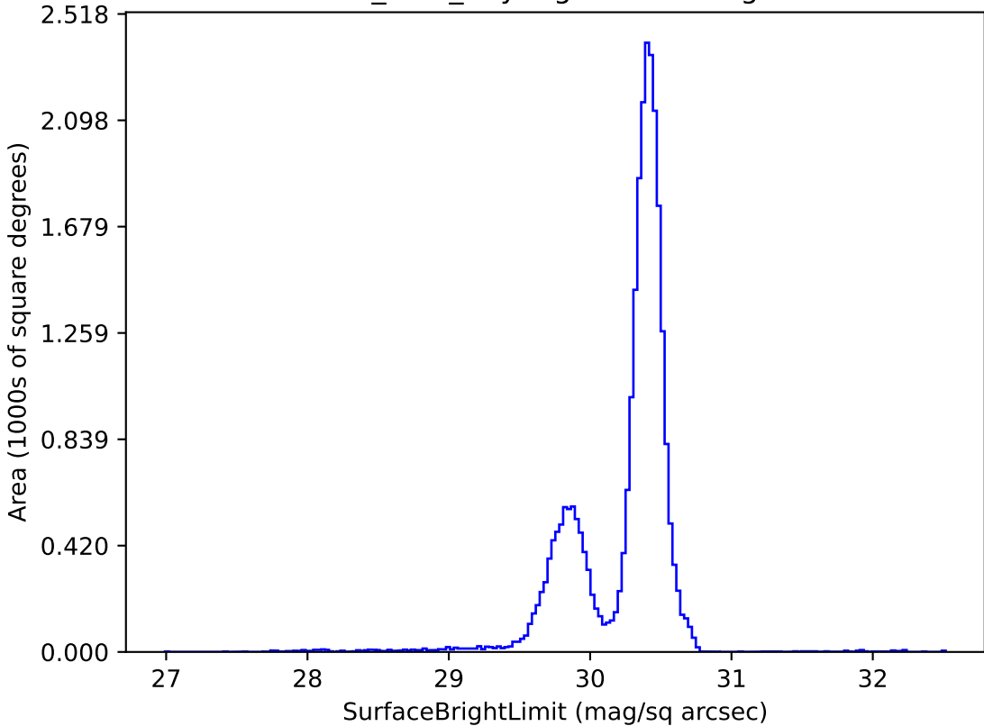
baseline_v3.4_10yrs g: SurfaceBrightLimit
