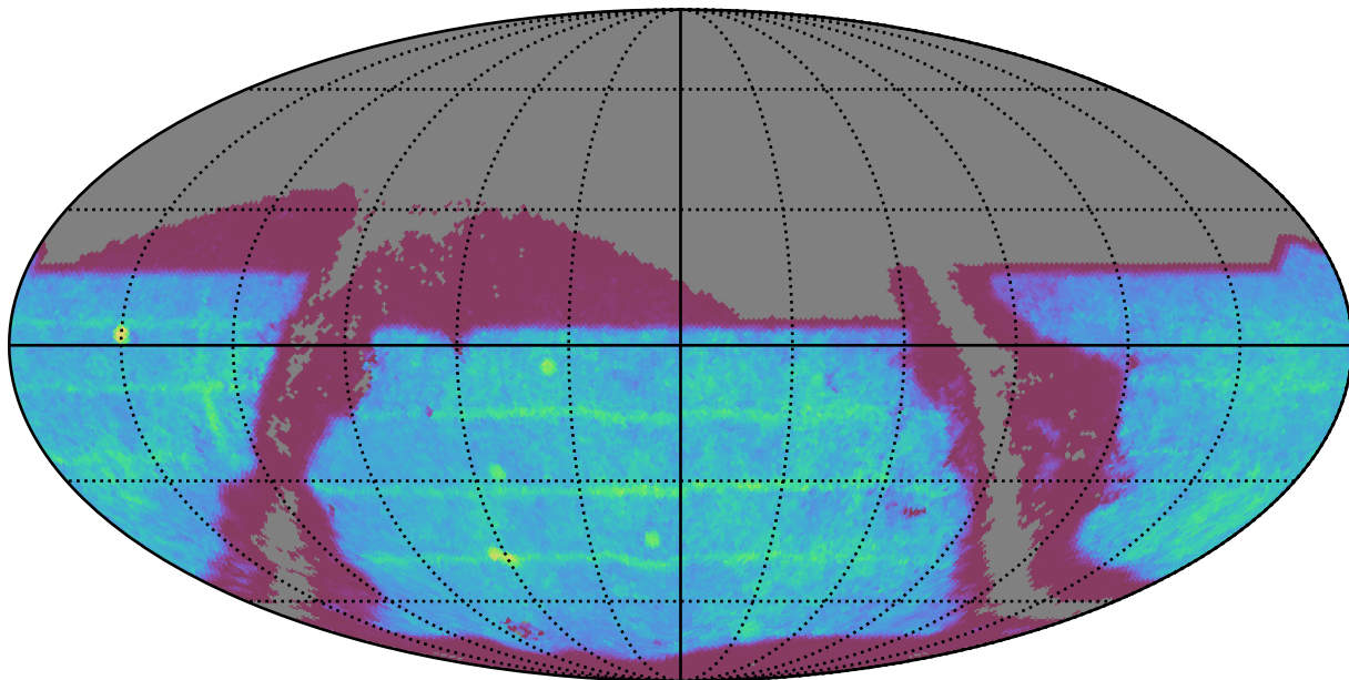
baseline_v3.4_10yrs : SNSLMetric
