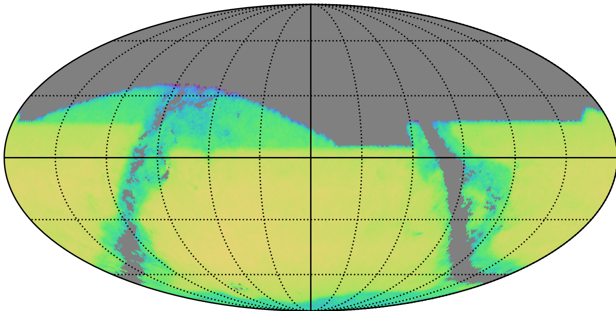
baseline_v3.4_10yrs z band and non-DD: QSONumberCountsMetric
