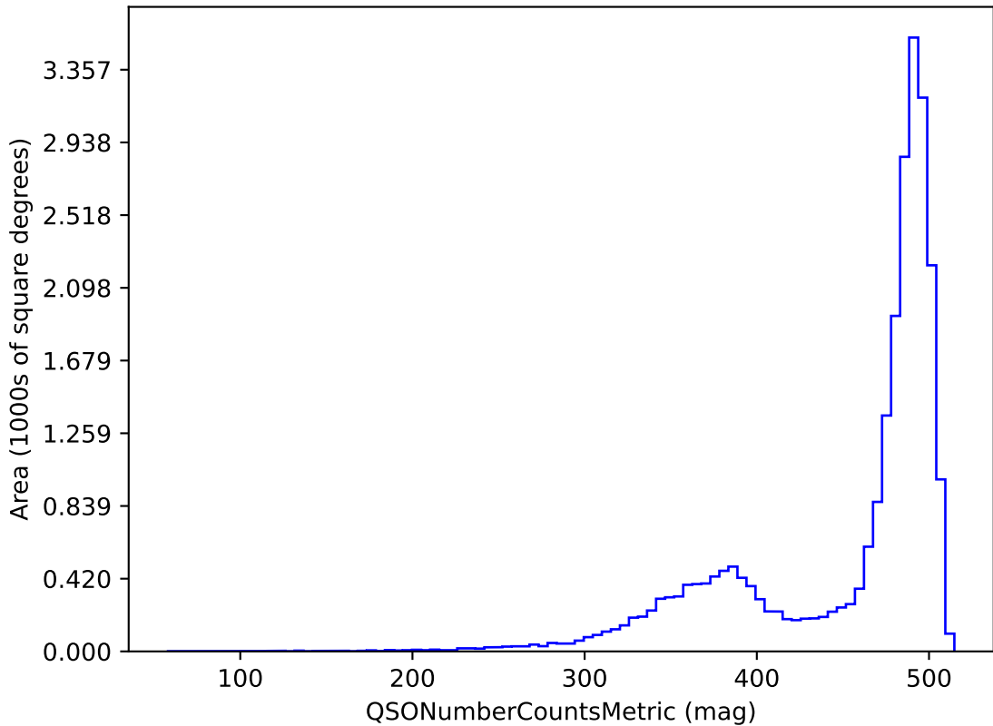
baseline_v3.4_10yrs z band and non-DD: QSONumberCountsMetric
