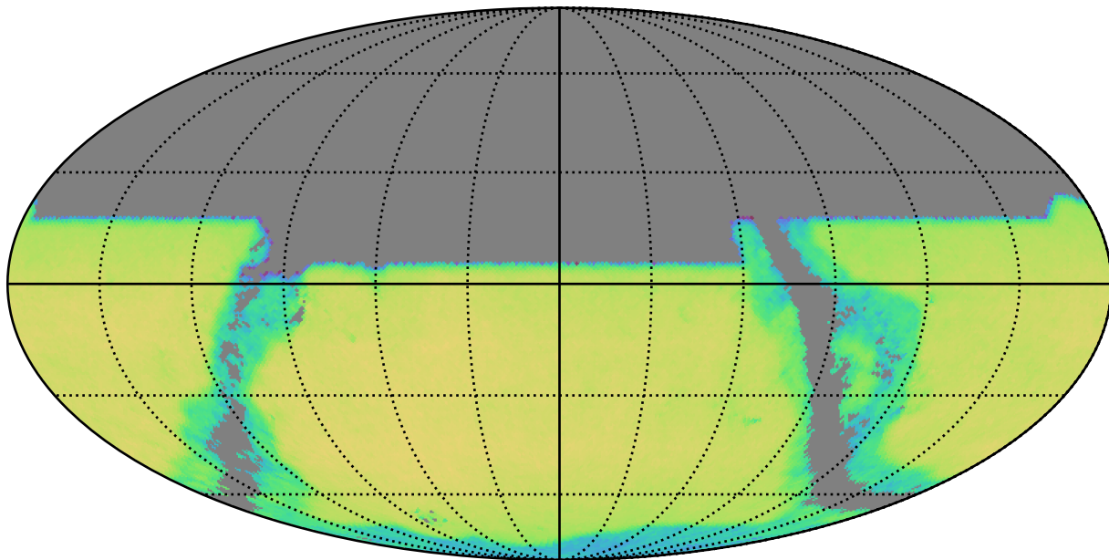
baseline_v3.4_10yrs y band and non-DD: QSONumberCountsMetric
