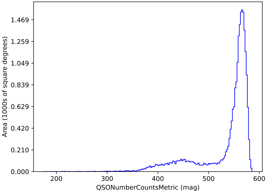
baseline_v3.4_10yrs y band and non-DD: QSONumberCountsMetric
