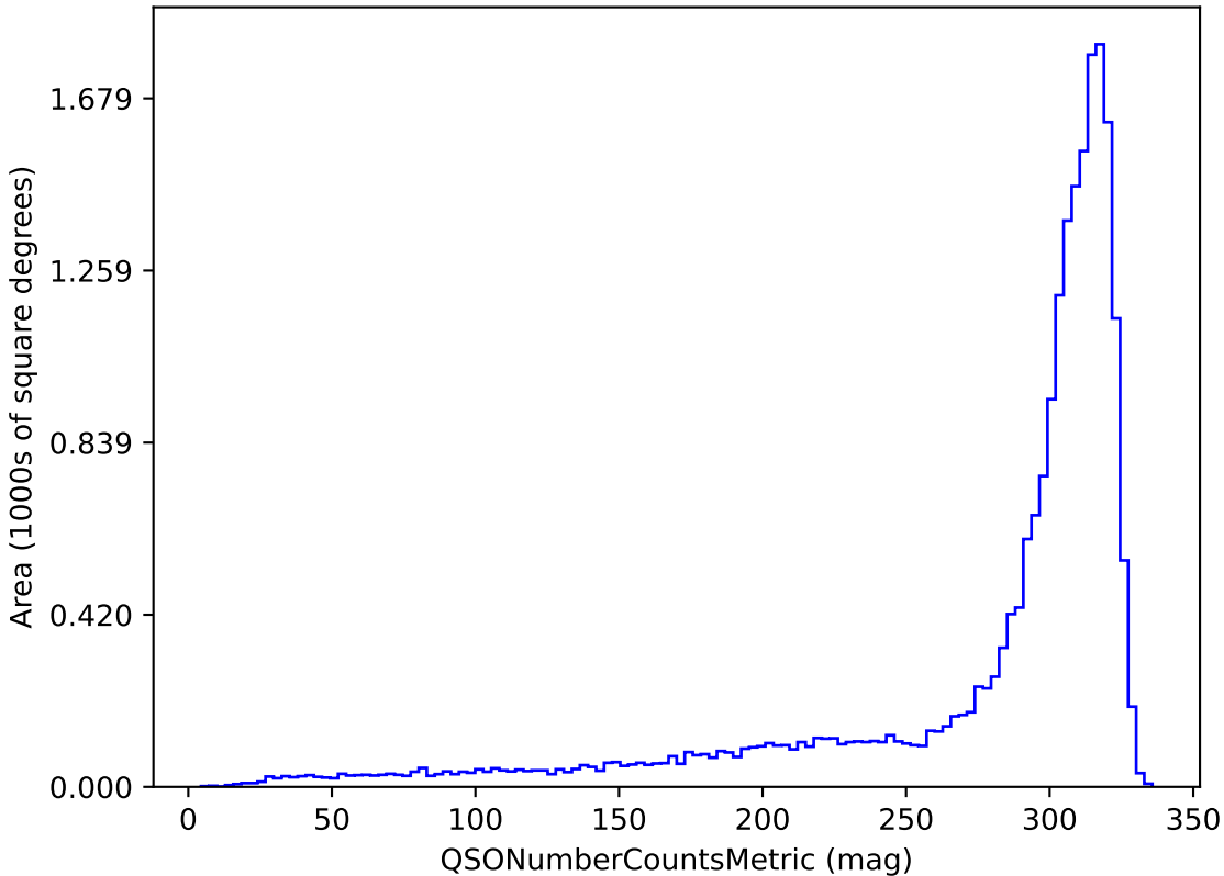
baseline_v3.4_10yrs u band and non-DD: QSONumberCountsMetric
