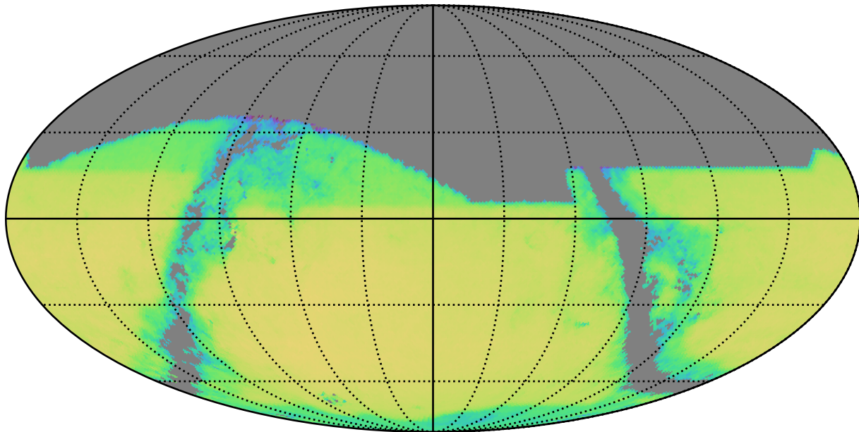
baseline_v3.4_10yrs r band and non-DD: QSONumberCountsMetric
