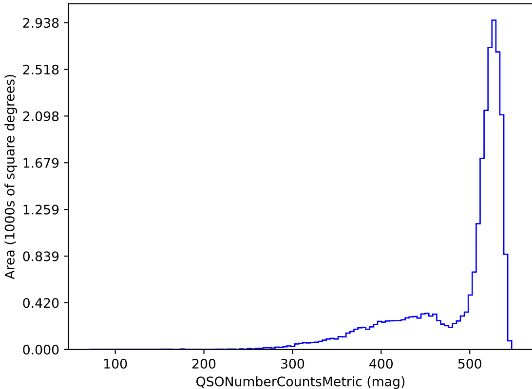
baseline_v3.4_10yrs r band and non-DD: QSONumberCountsMetric
