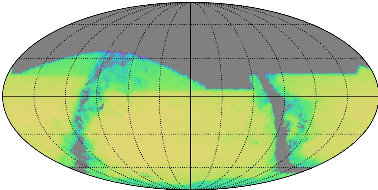
baseline_v3.4_10yrs i band and non-DD: QSONumberCountsMetric
