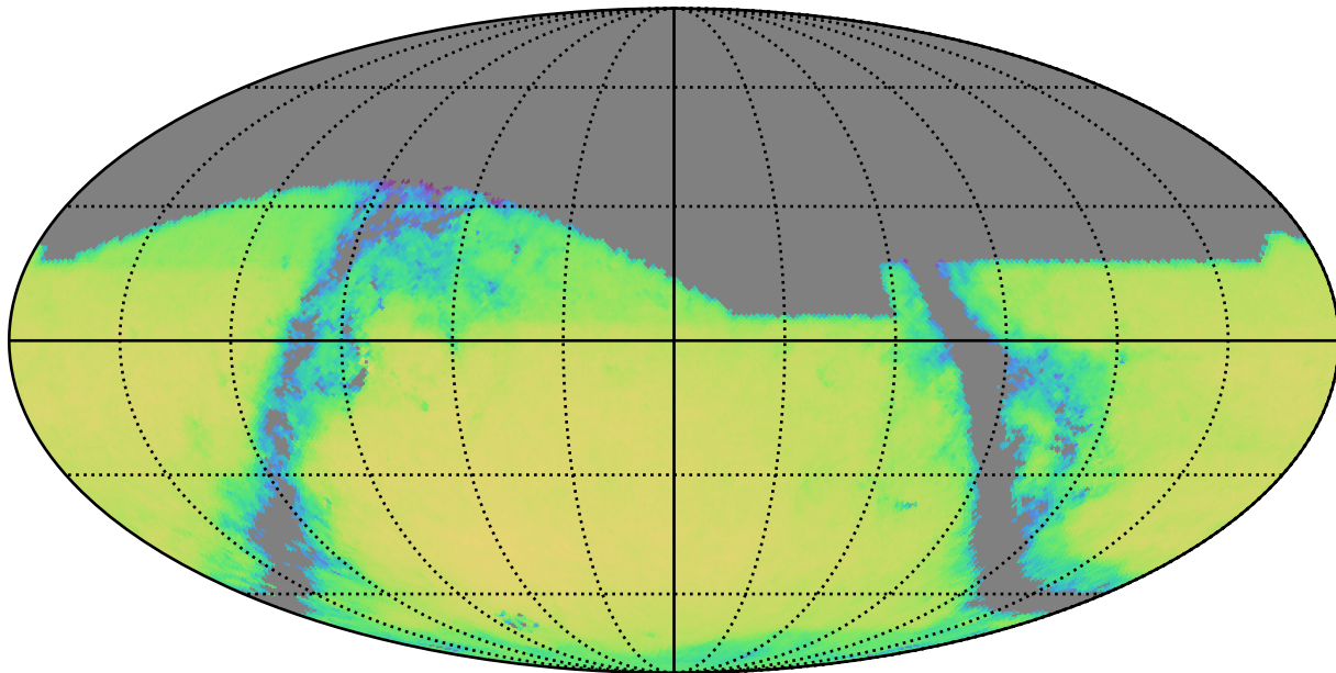
baseline_v3.4_10yrs g band and non-DD: QSONumberCountsMetric
