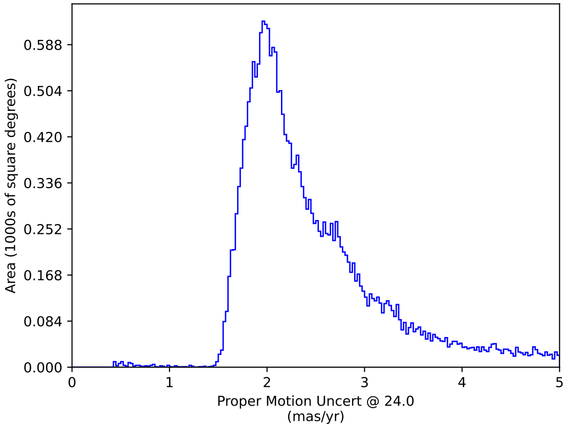
baseline_v3.4_10yrs : Proper Motion Uncert @ 24.0
