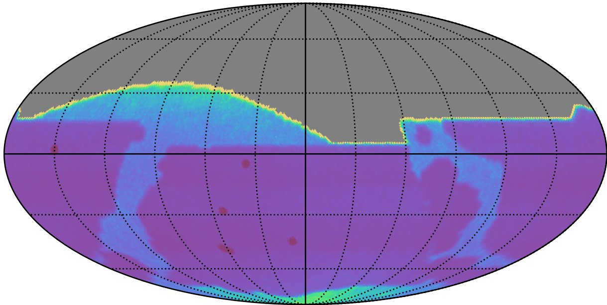
baseline_v3.4_10yrs : Proper Motion Uncert @ 20.5
