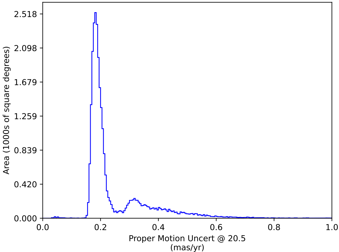
baseline_v3.4_10yrs : Proper Motion Uncert @ 20.5
