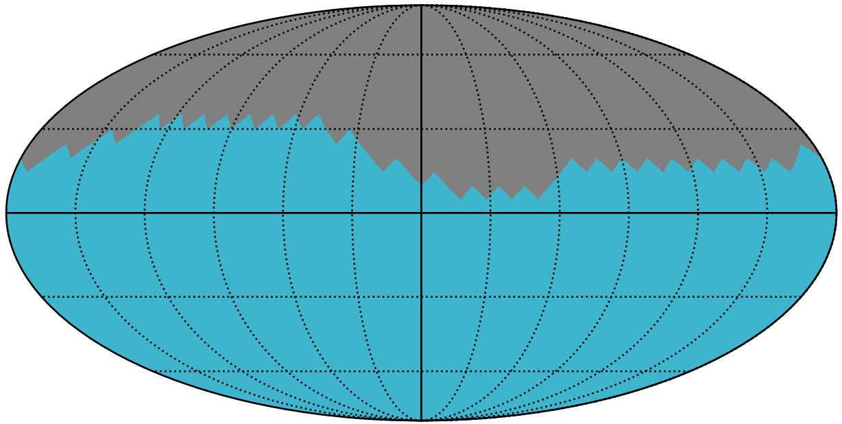
baseline_v3.4_10yrs dm 20 interval 30 RRc Year 1-2: PeriodicStarModulationMetric
