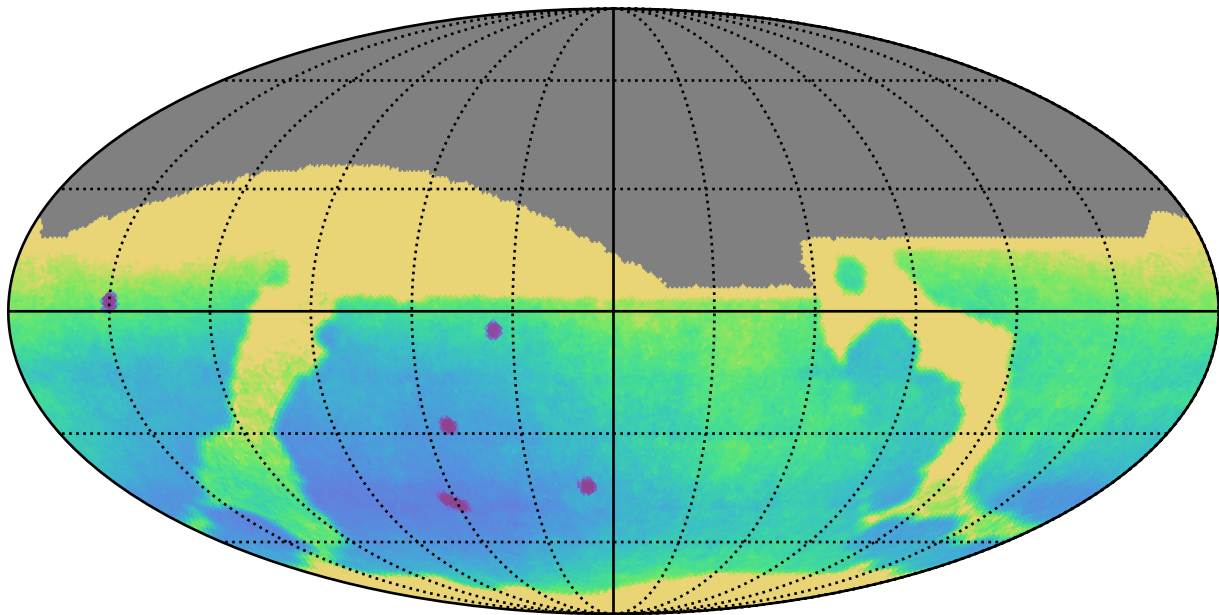
baseline_v3.4_10yrs : Parallax Uncert @ 24.0
