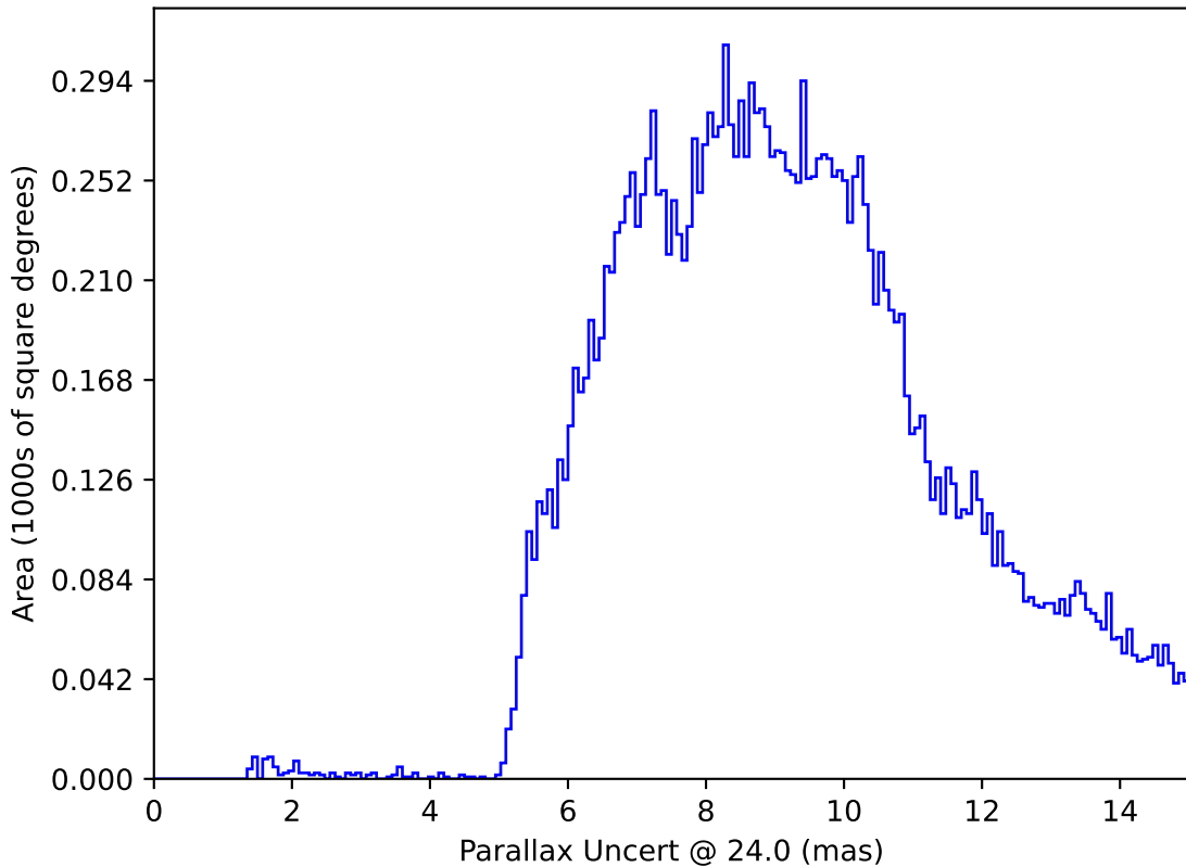
baseline_v3.4_10yrs : Parallax Uncert @ 24.0
