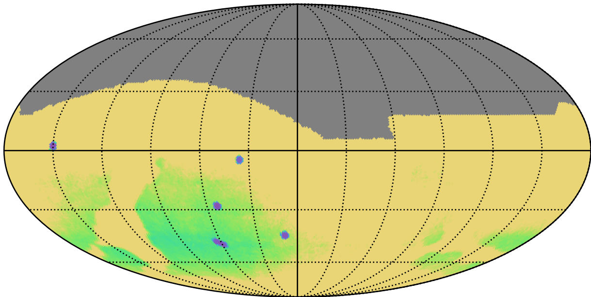
baseline_v3.4_10yrs : Parallax Uncert @ 22.4
