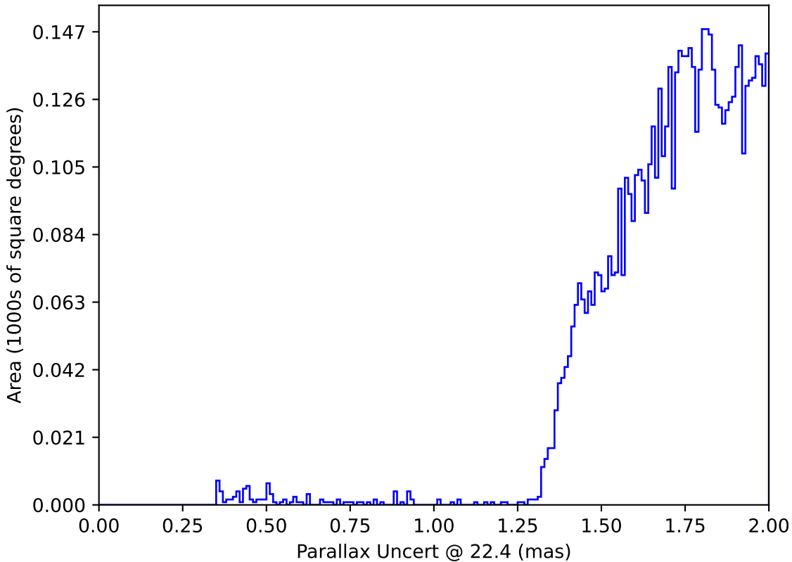
baseline_v3.4_10yrs : Parallax Uncert @ 22.4
