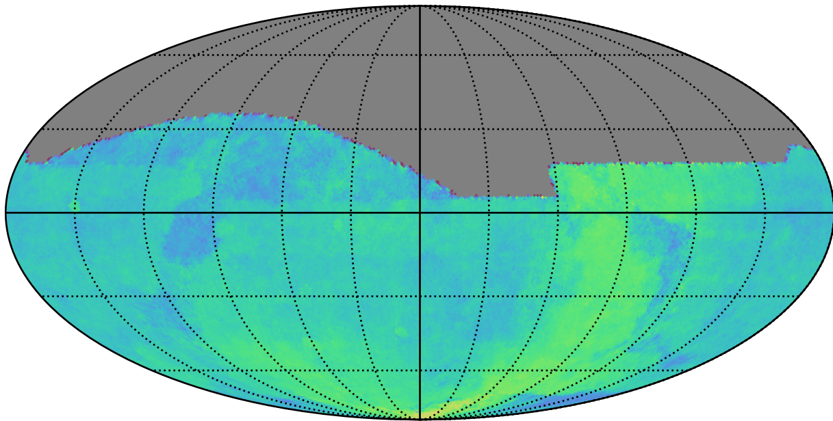
baseline_v3.4_10yrs : Parallax Coverage @ 24.0
