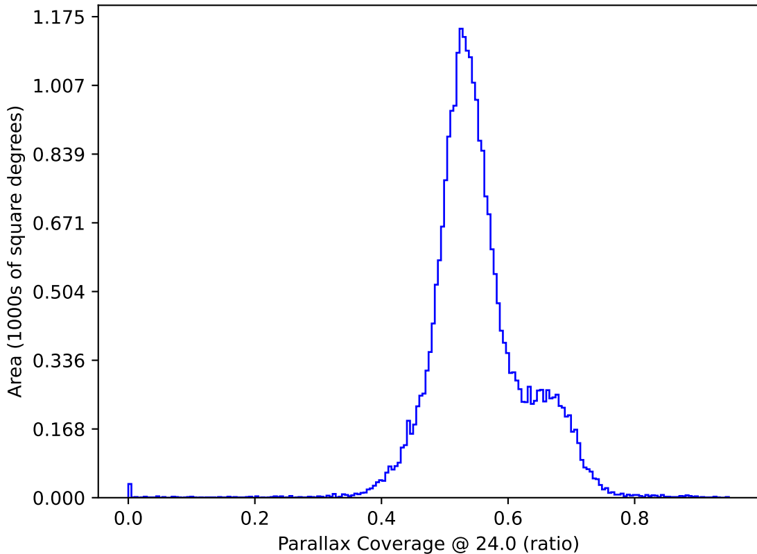
baseline_v3.4_10yrs : Parallax Coverage @ 24.0
