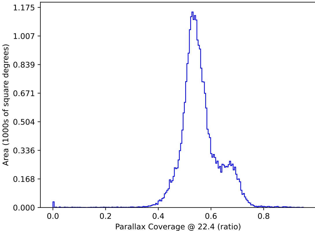
baseline_v3.4_10yrs : Parallax Coverage @ 22.4
